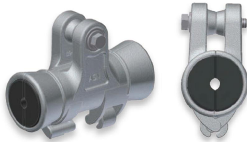
Figure 4 ADSS Suspension clamp housing showing the bushing
